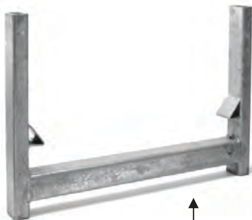
VMT 100800 - U-frame
